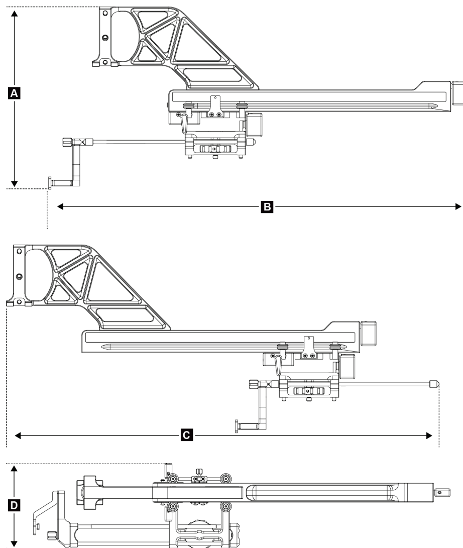
Figur 74: Lateral arm
