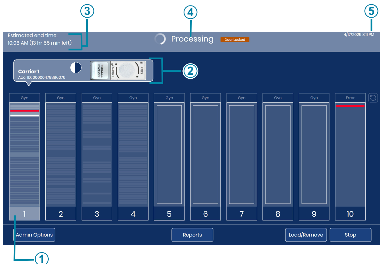
Figure 3-5 Screen Display During Processing
