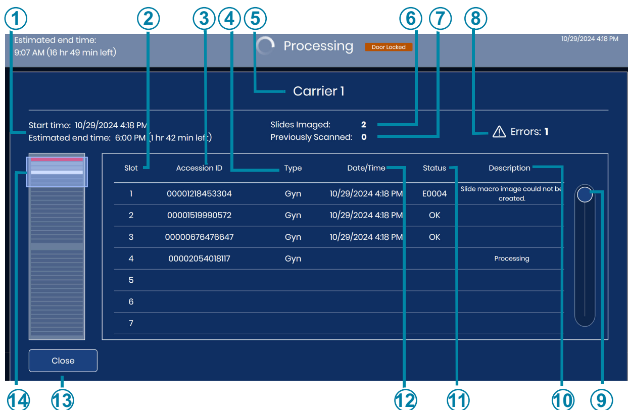
Figure 3-7 Slide Carrier Details Screen (Carrier 1, example)
