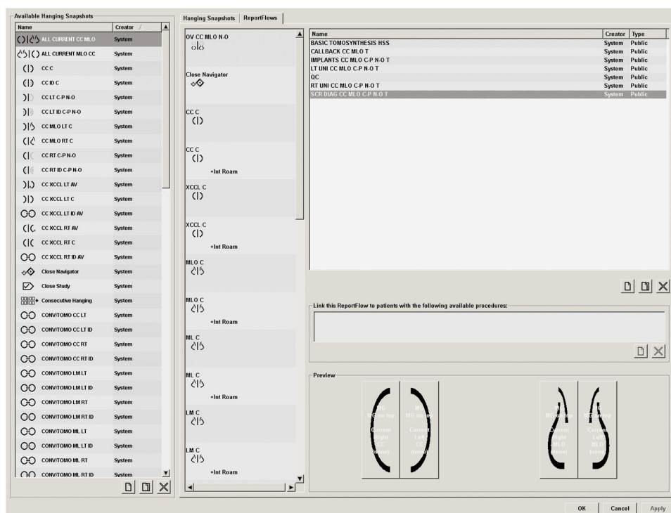
Figura 98: Fila ReportFlows
