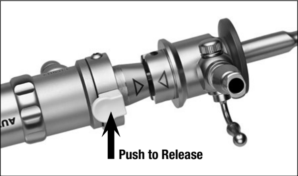
FIGURE 2. SECURE SHEATH
