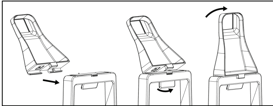
Figure 59: How to Install a Compression Paddle
