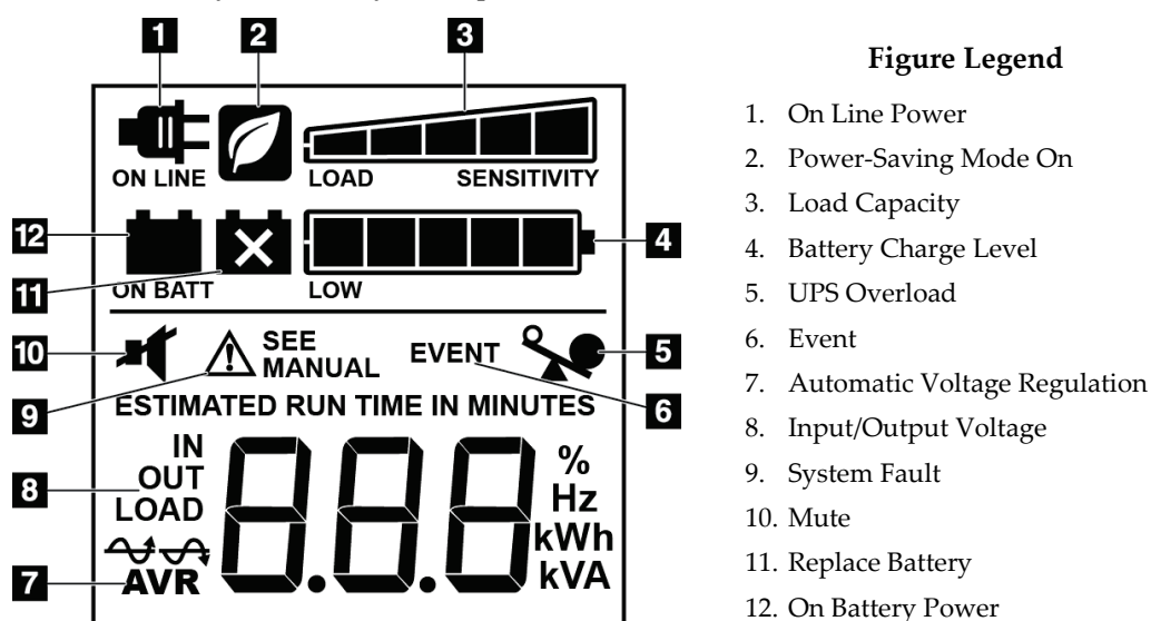
Figure 83: UPS LCD Display
