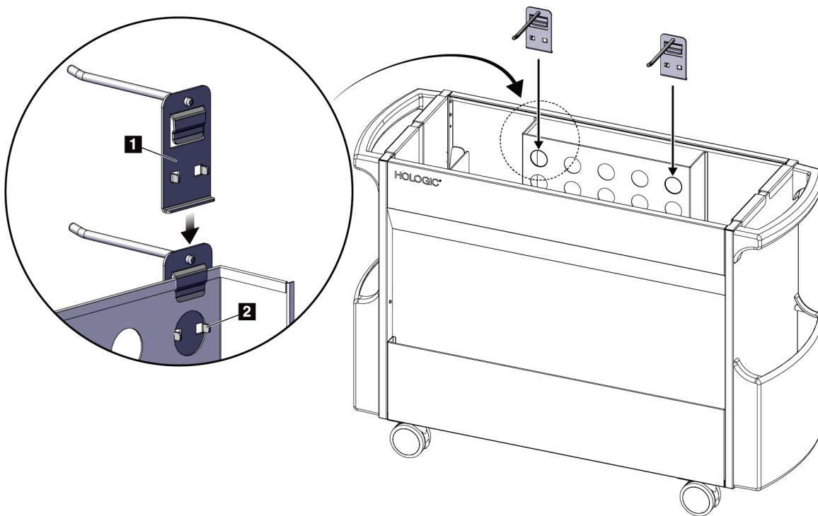
Figure 63: Pad Hanger Installation
